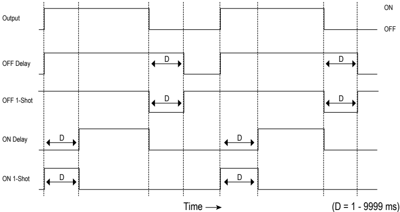
Figure 3. DF-G1 Delays/Timers
